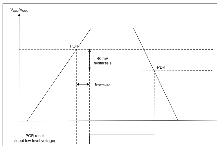
Figure 2-3 POR/PDR thresholds
