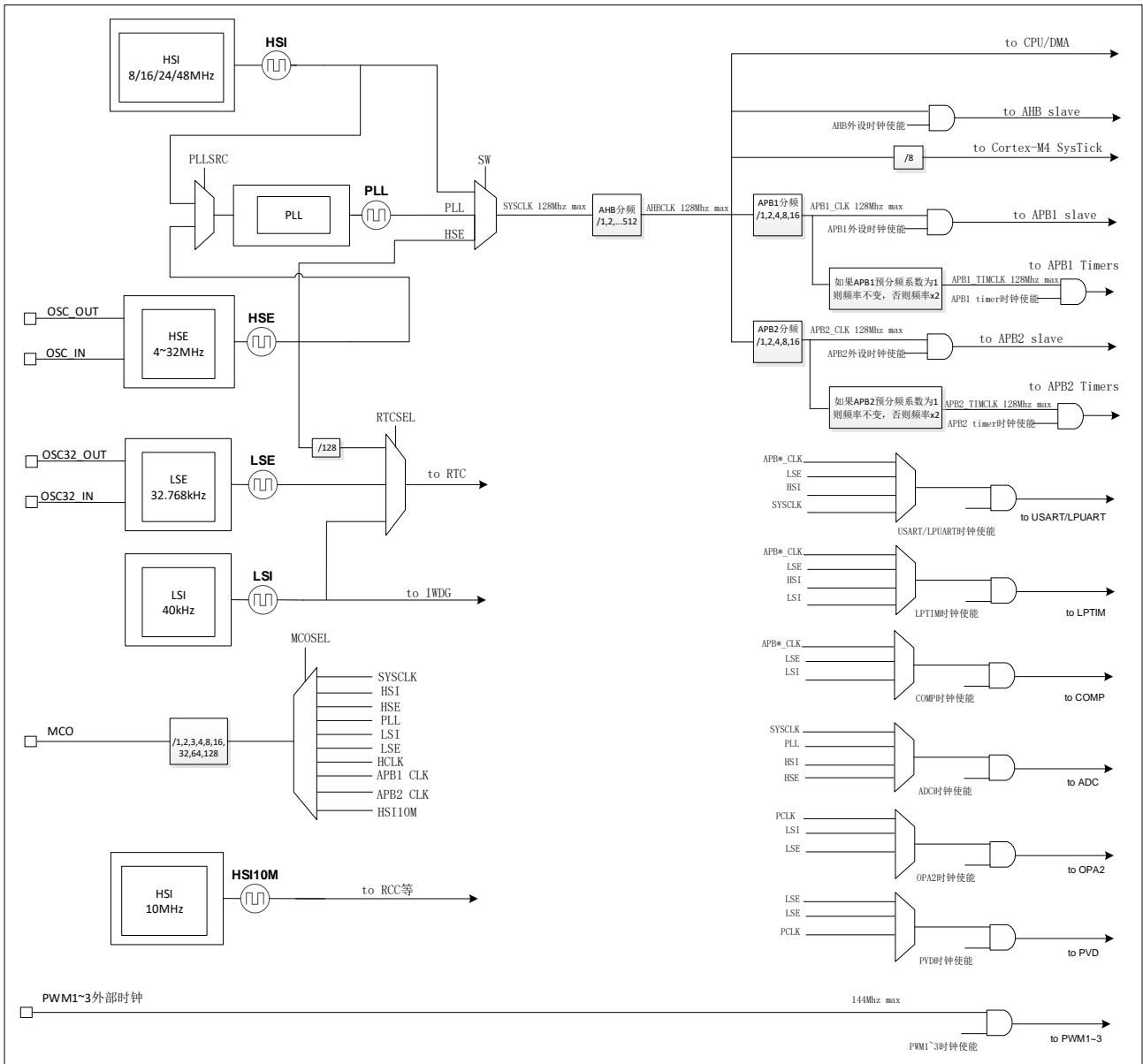
Figure 2-1 System clock structure diagram
