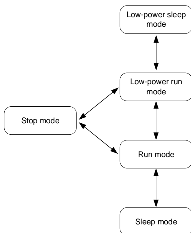
Figure 2-5 Low-power mode
