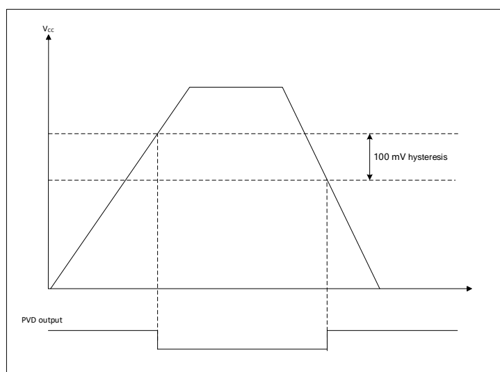
Figure 2-4 PVD threshold
