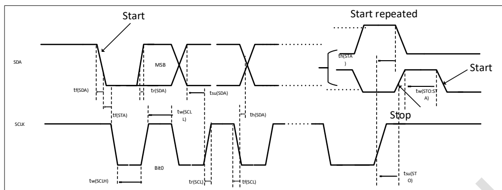
Figure 5-4 I 2 C bus timing diagram
